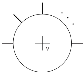
Figure 1: Tadpole calculation of superpotential
